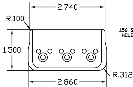
TOP VIEW PLATE DIMENSIONS
