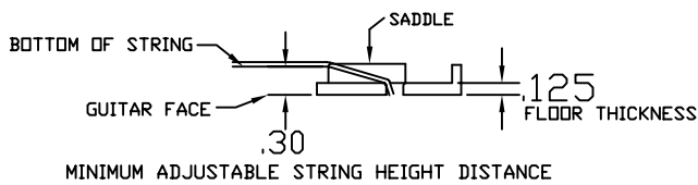
SIDE VIEW OF 41100
