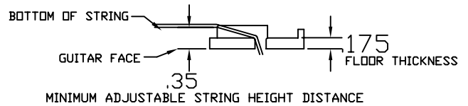
SIDE VIEW OF 41105
