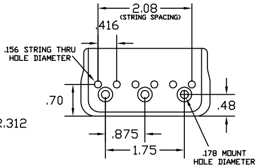
TOP VIEW HOLE PATTERN DIMENSIONS
